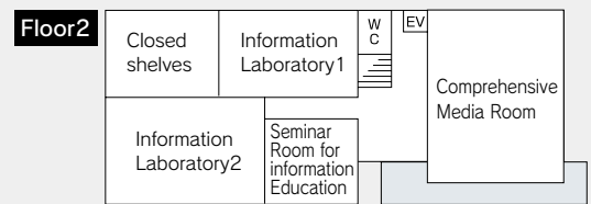
Floor layout
